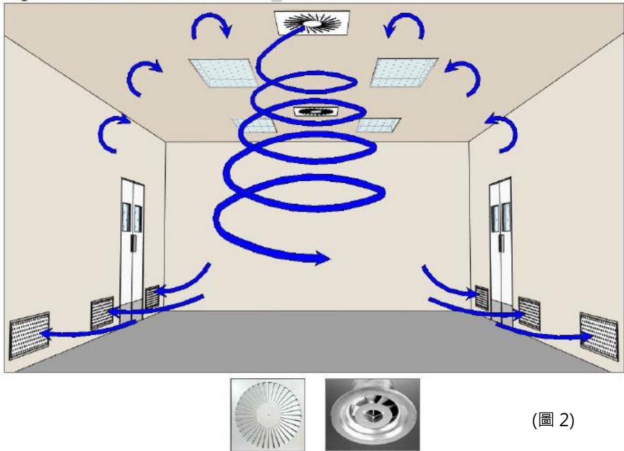
Figure 20. Swirl diffuser
